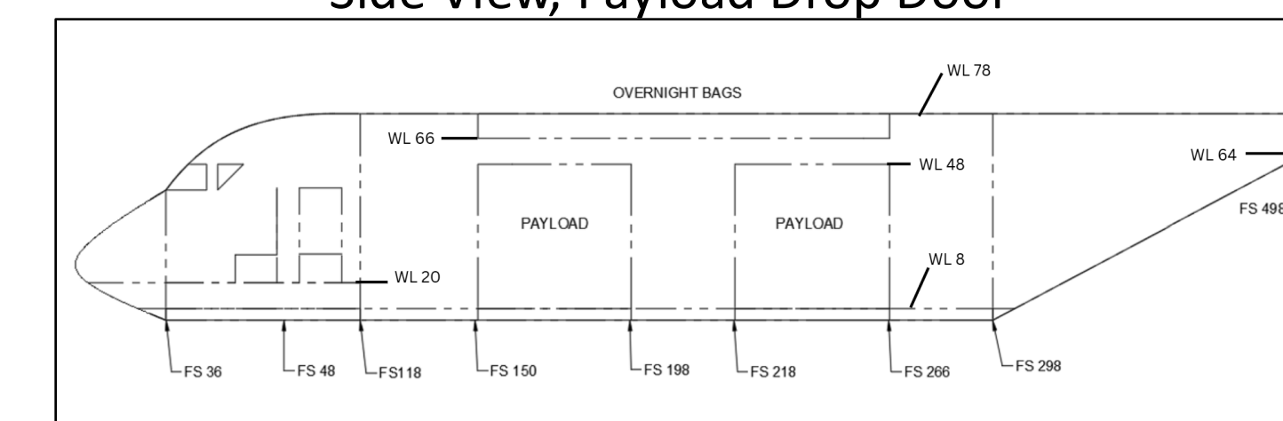
Side View, Overall
