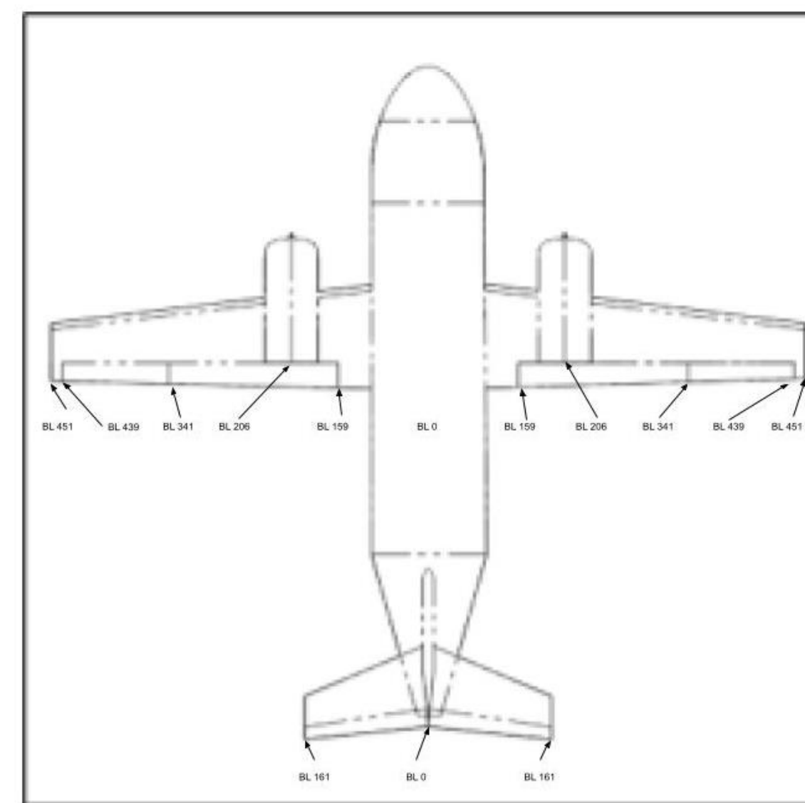
Top View, Overall
